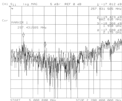
Graph 3: Cable return loss NS100TRI - port 1
